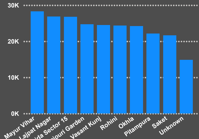
Top 10 Pickup Location By Total fare
